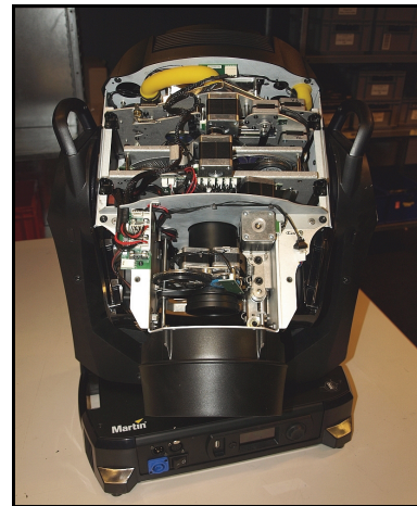
Figure 13: Head positioned for service access
