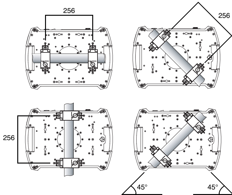
Figure 2: Clamp bracket positions
