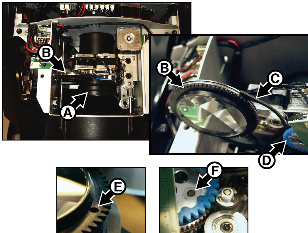
Figure 16: Prism removal and installation
