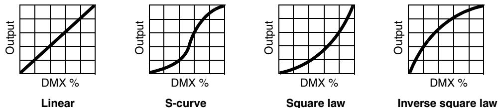
Figure 5: Dimming curve options
