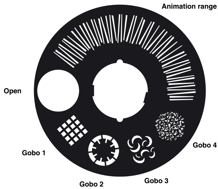
Figure 2: Super Sic 58 FX wheel
