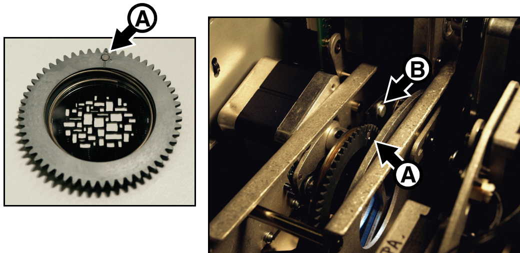
Figure 18: Goboholder position for replacement
