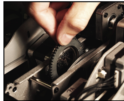
Figure 19: Gobo removal
