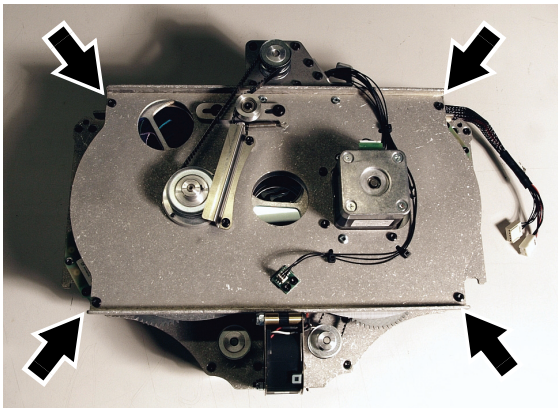
Figure 26: Opening the projection module
