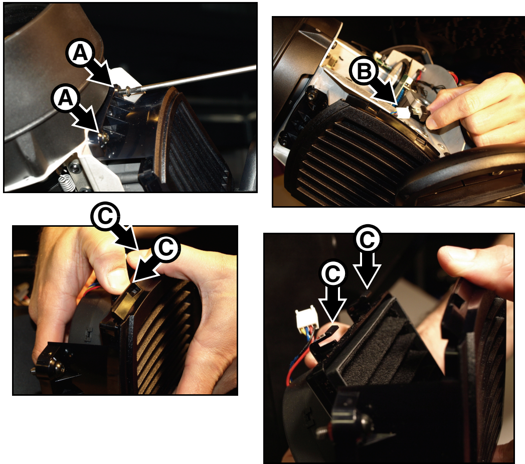
Figure 14: Head air filter removal
