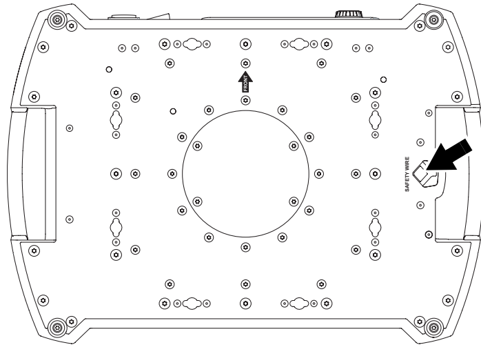
Figure 6: Safety cable attachment point
