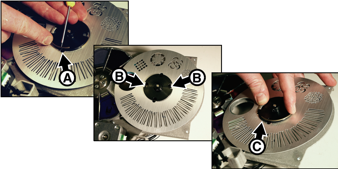
Figure 27: FX wheel removal and mounting
