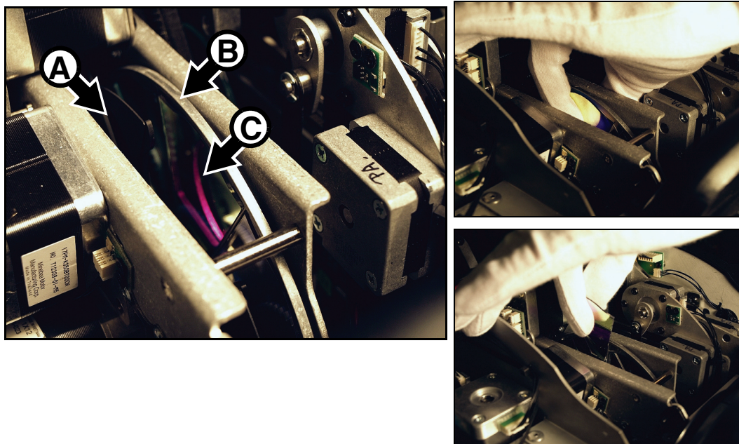
Figure 22: Color filter removal
