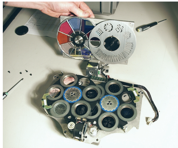
Figure 26: Opening the projection module
